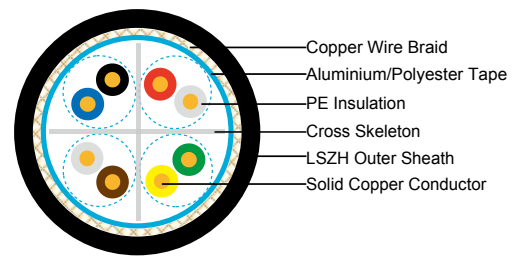
SF/UTP CAT6
